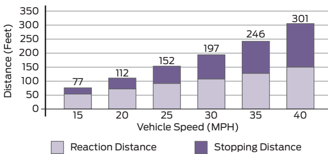
Reaction & Stopping Distance vs. Speed
